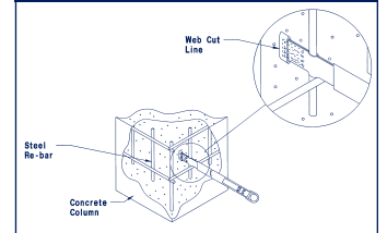
Figure 9 - Anchorage Connector Installed
