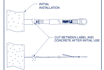
Figure 8 - Anchorage Connector Installed
