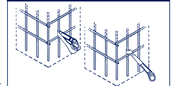
Figure 7 - Installing in Second Location
