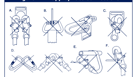
Figure 4 - Inappropriate Connections
