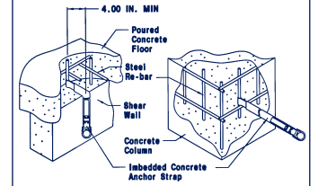
Figure 6 - Installing On Completed Cage
