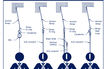
Figure 9 - Anchorage Connector Installed
