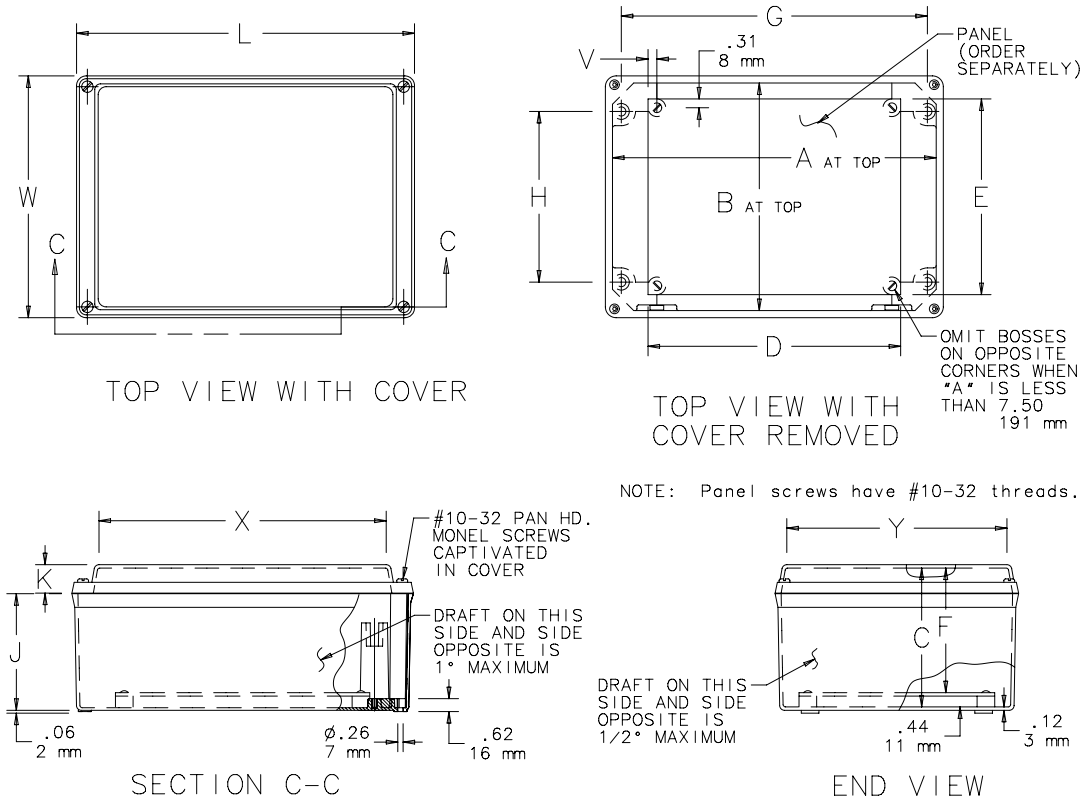
Solid Screw Cover Enclosure
