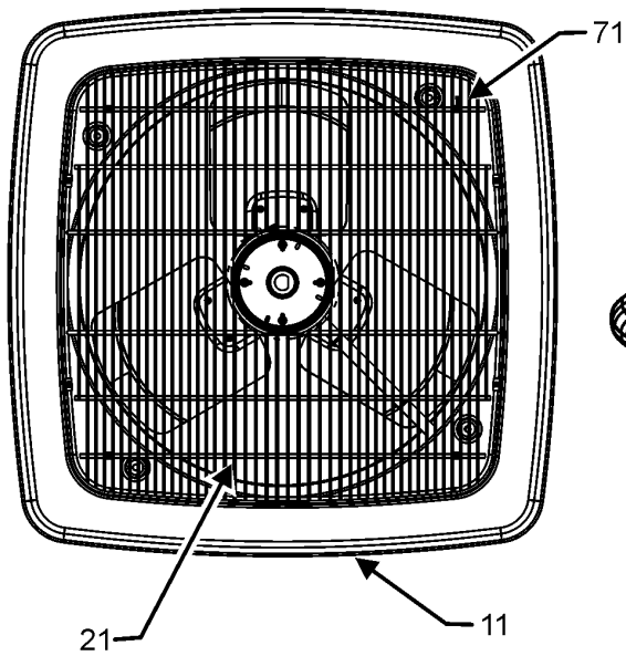
TOP PANEL ASSEMBLY TOP VIEW
