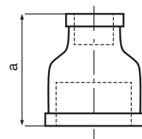
Red. Coupling - Dimensions
