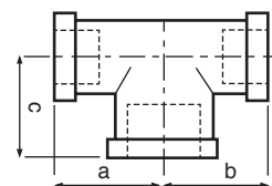
Bull Head Tees - Dimensions
