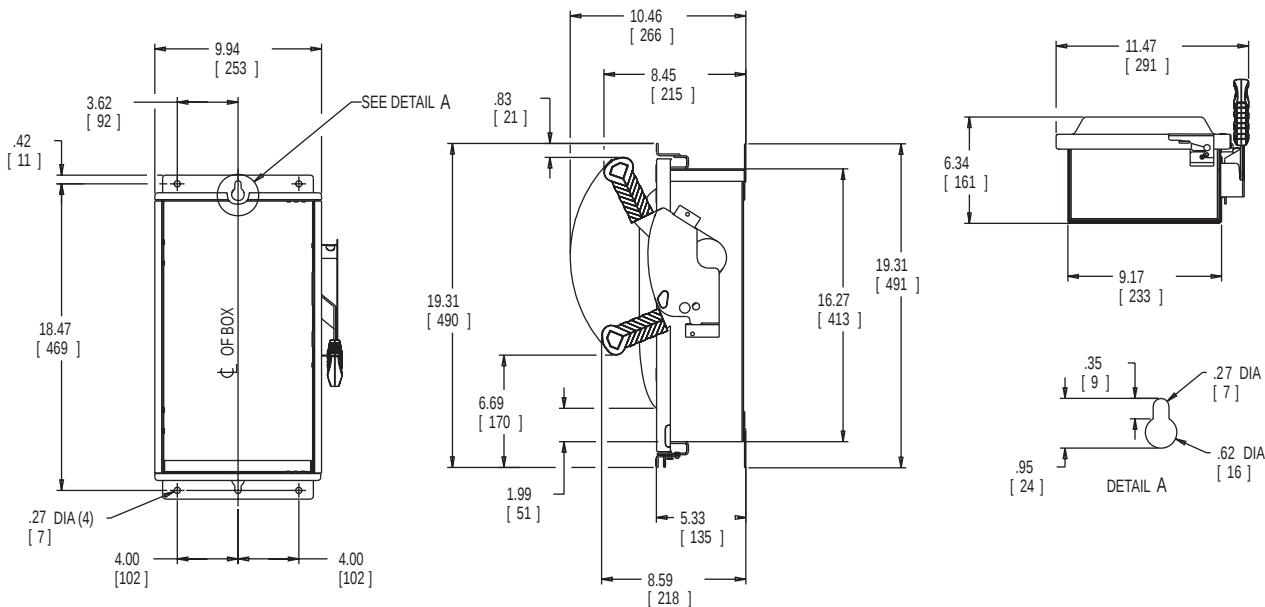
100 Amp Heavy Duty
