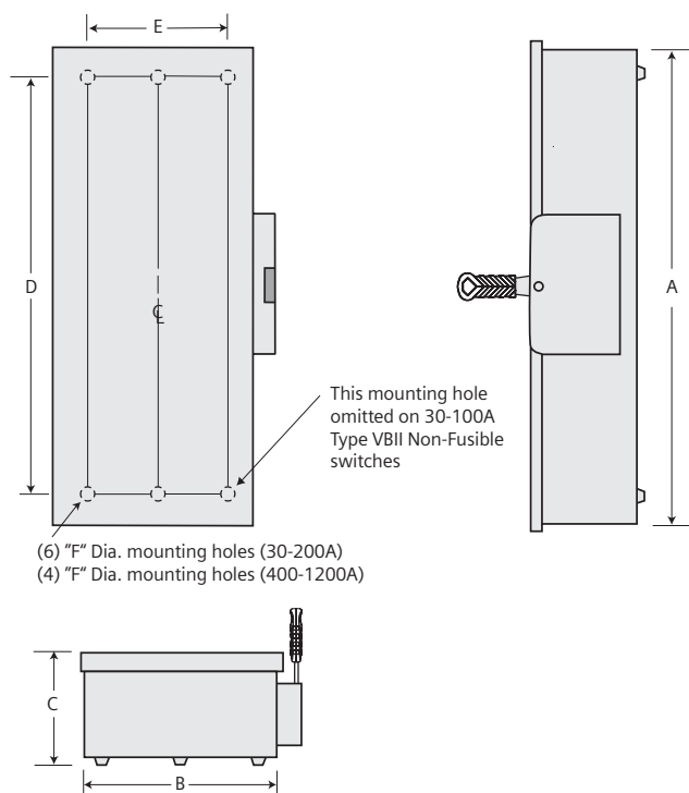
Figure 1: Type 1 & 3R ④
