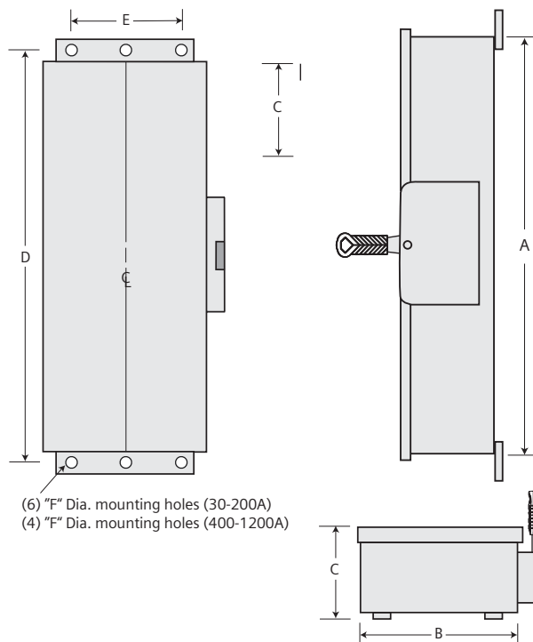
Figure 2: Type 4X &amp; 12
