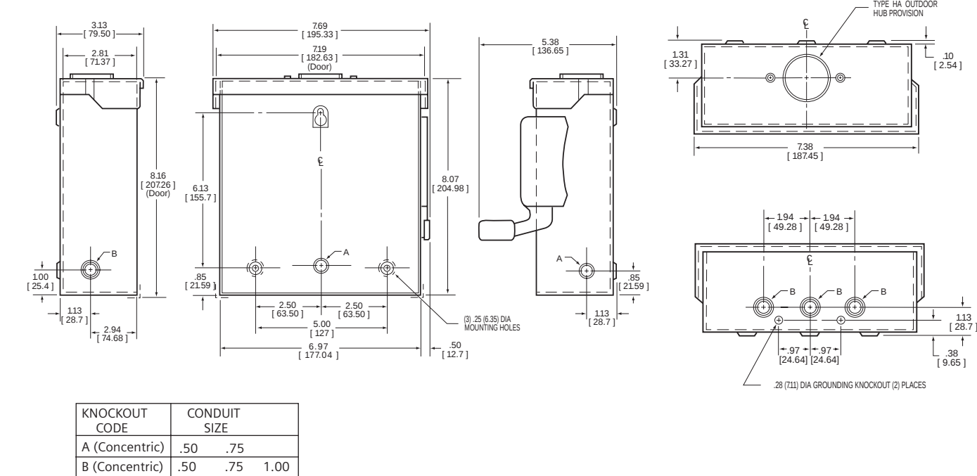
Type 3R (Outdoor) 30 Amp General Duty (3-Pole)
