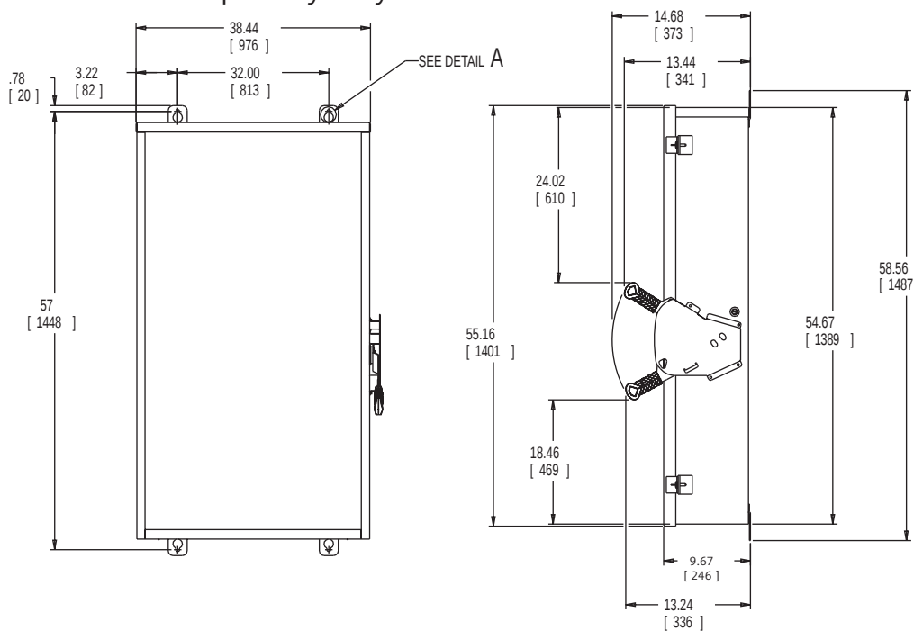
800 / 1200 Amp Heavy Duty Non-Fusible
