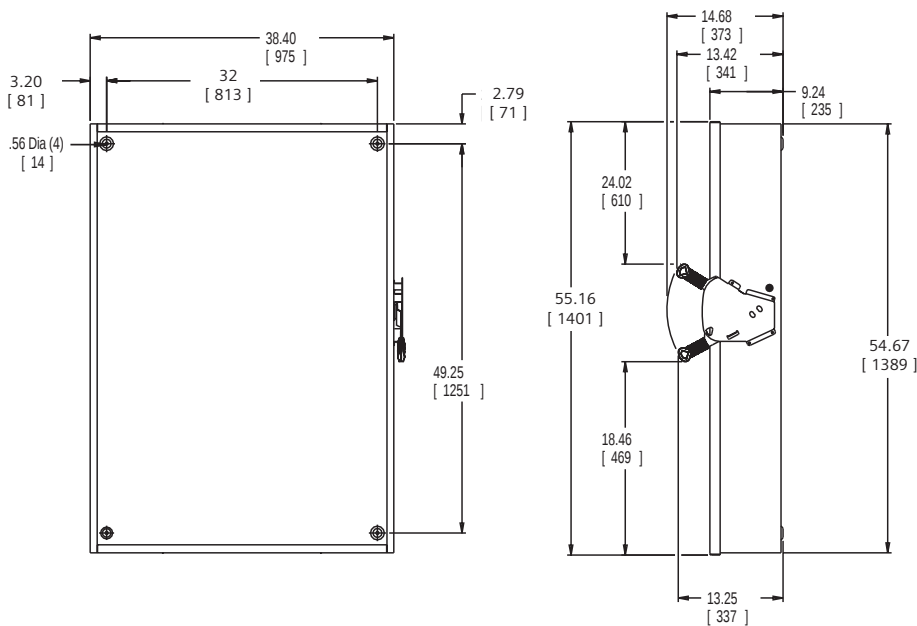
800 / 1200 Amp Heavy Duty Non-Fusible
