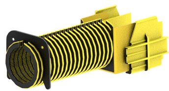
FiberGuide® Single 2" Flex Tube Attachment, 2 in x 2 in, 5 ft length, yellow
