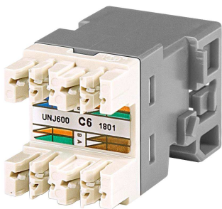
Uniprise Modular Jack, RJ45, category 6, T568A/T568B, unshielded, without dust cover, gray
