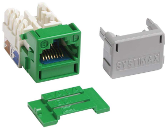
GigaSPEED X10D® MGS600 Series Information Outlet, green
