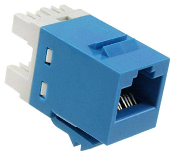
SL110 Series Modular Jack, 8-position, RJ45, category 5e, T568A/T568B, unshielded, without dust cover, blue
