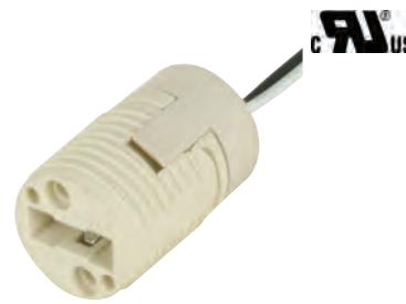
80-1500 Phenolic Socket 20" UL 10362 B/W Leads 1/8 IP Bushing 1 1/4" H x 3/4" Dia. 500W-250V
