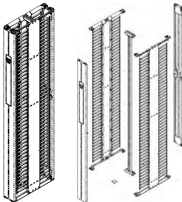
Motive Double-Sided Vertical Cable Manager P/N 32620-XXX
