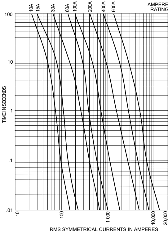
AVERAGE TIME/CURRENT CURVES Cat No. ECSR (AMP) 600 VAC
