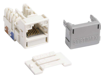
GigaSPEED XL® MGS400 Series Category 6 U/UTP Information Outlet, white
