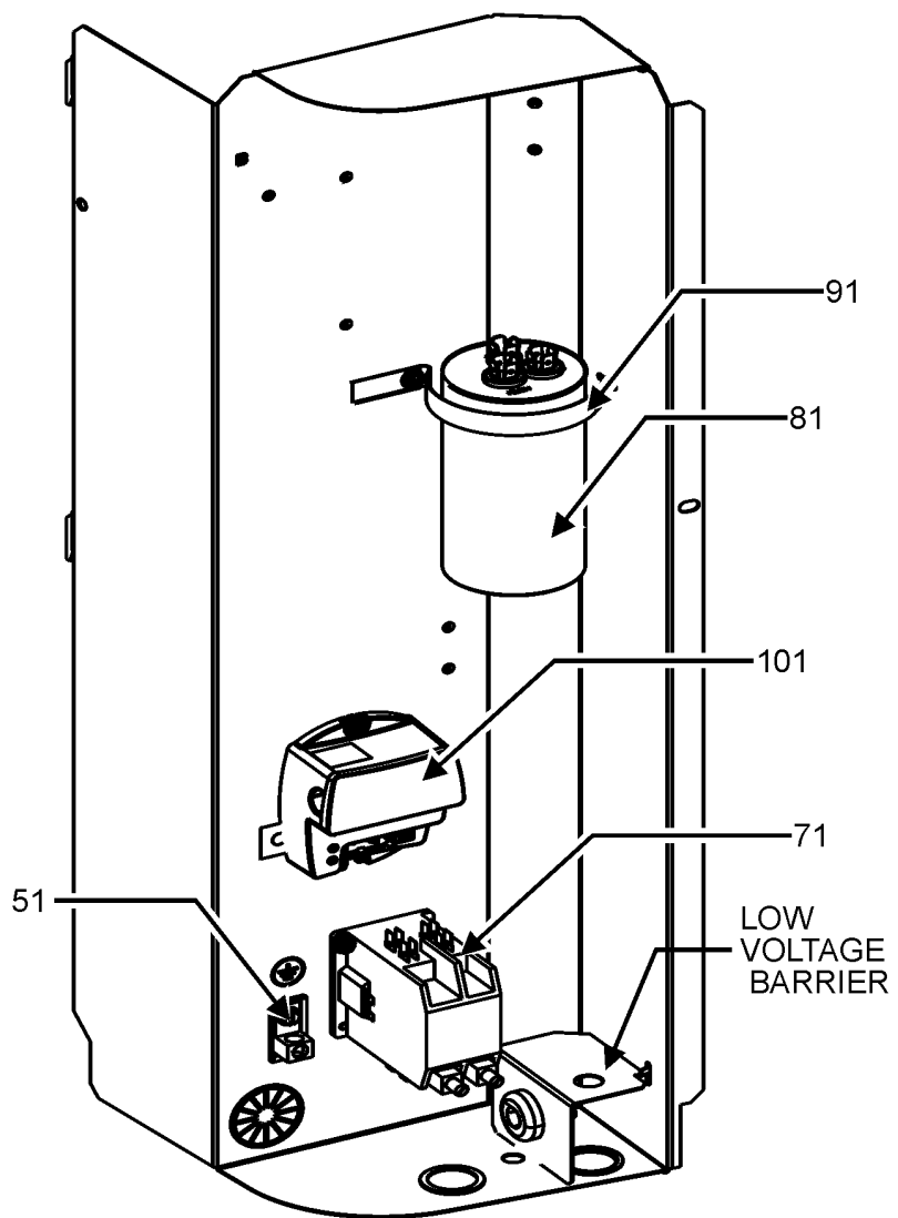
CONTROL PANEL
