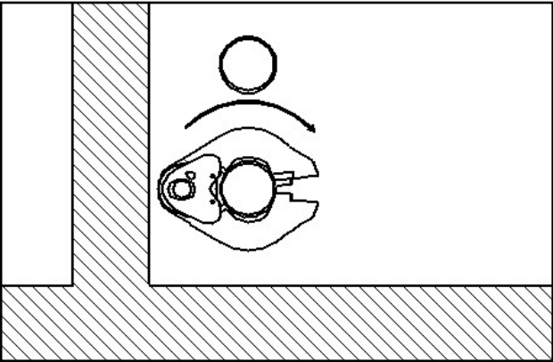
3. Keep the press ring closed and rotate about the fitting until the opening is toward the front
