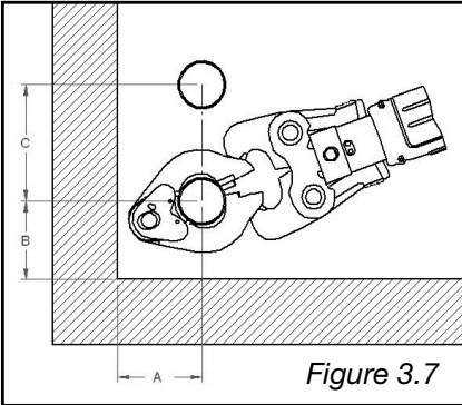
4. Insert the press ring actuator and start the press cycle
