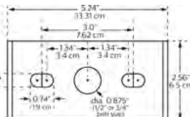
Trunnion Mount Bolt Pattern
