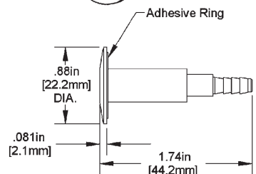
Low Profile Port
