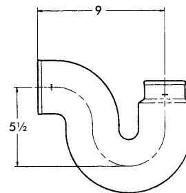
REDUCING P-TRAP
