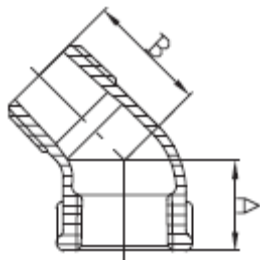
45 Street Elbow
