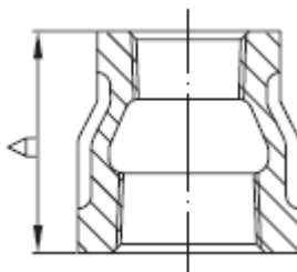
Reducing Coupling
