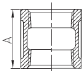
Coupling
