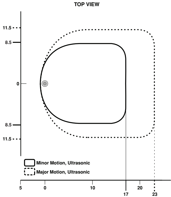
Figure 2 (Cat. No. OSC05) Field-of-View Ranges
