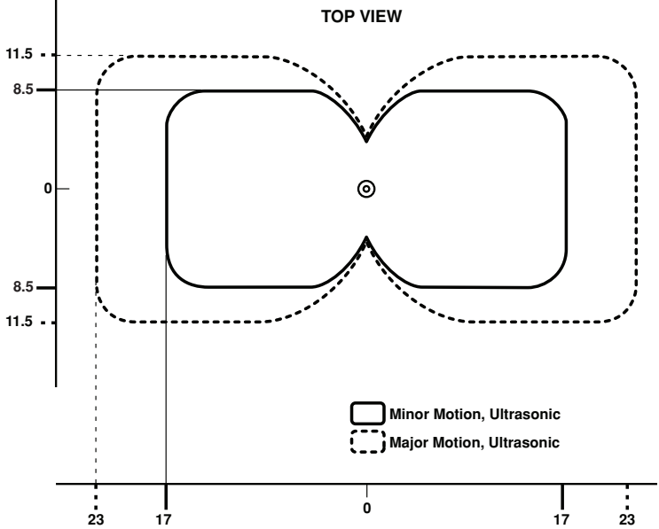
Figure 3 (Cat. No. OSC10) Field-of-View Ranges
