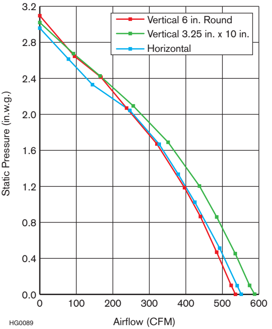
Airflow Performance at High Speed
