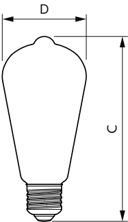
ST19 5.5-60W 500lm 2700-2200K E26 D CL
