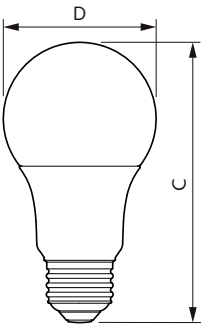
Bulb A19 120V 5-40W 450lm 5000K E26 D
