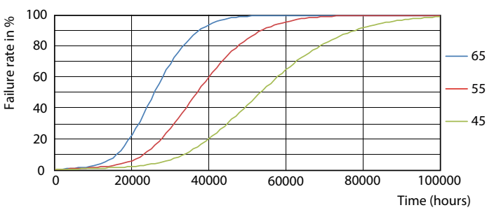
LEDtube FA8 4000K 240D FailureRate
