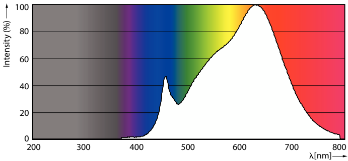
Spectral Power Distribution Colour - 8.5PAR20/PER/930/F25/DIM/EC/120V 6/1FB
