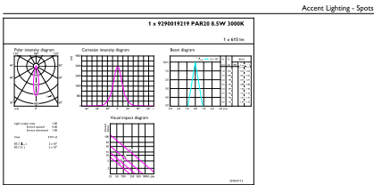
Light Distribution Diagram - 8.5PAR20/PER/930/F25/DIM/EC/120V 6/1FB
