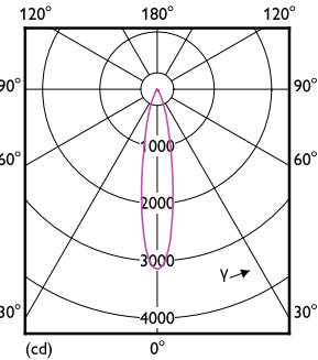
Light Distribution Diagram - 8.5PAR20/PER/930/F25/DIM/EC/120V 6/1FB
