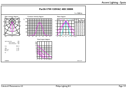
PAR38 120V 17-120W 40D 3000K E26 D
