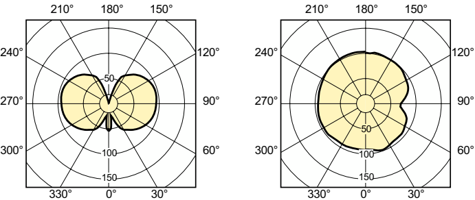
Light Distribution Diagram - MASTERColor CDM-T Elite 35W/930 G12 1CT
