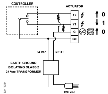
Figure 8 For Triac Driven Controllers, (TEC, DXR, and Others).
