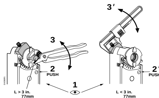
Figure 14. Manual Override.
