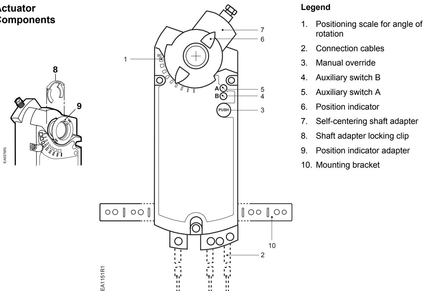
Figure 11. Components of the 3-Position Actuator.
