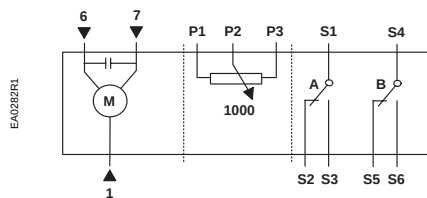
Figure 21. 24 Vac with Auxiliary Switches.
