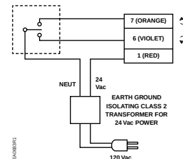
Figure 22. 24 Vac, 3-Position Control.
