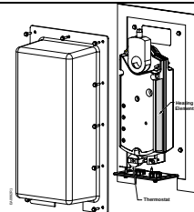
Figure 8. Heater/Weather Shield Assembly.
