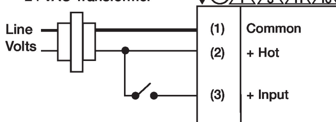
Floating Point - Triac Source
