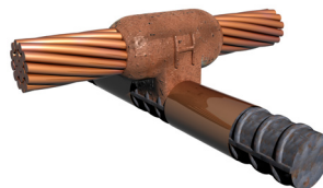
(Cross of Horizontal Cable Lapped Over Horizontal Rebar)
