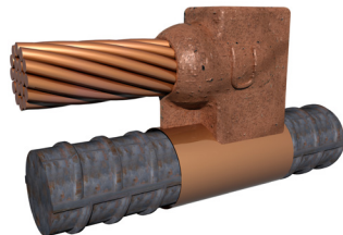
(Parallel Cable Tap of Horizontal Cable to Thru Horizontal Rebar)
