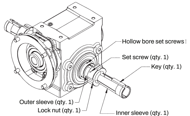
Figure 14 - Grip Tight Bushing Kit
