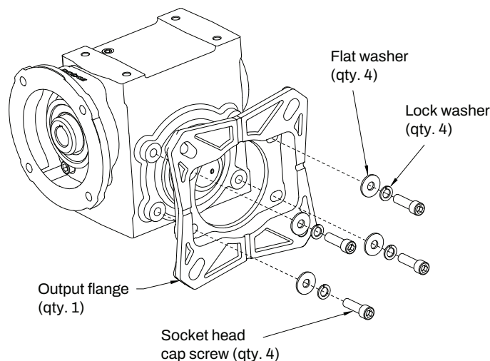
Figure 4 - Output Flange Kit
