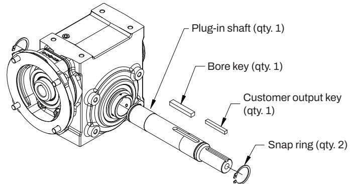
Figure 11 - Plug-in Shaft Kit
