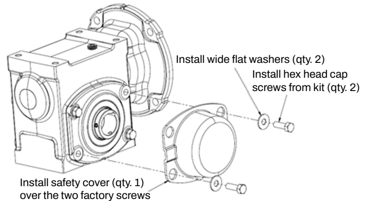
Figure 7 - Installation on Bearing Cover Side
