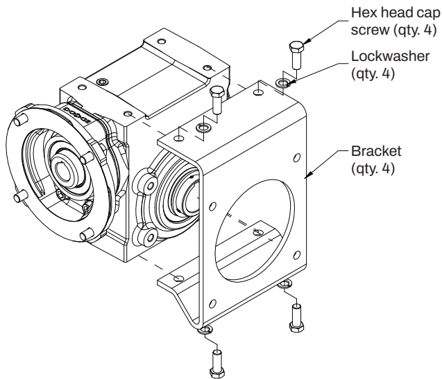
Figure 5 - Output Bracket Kit
