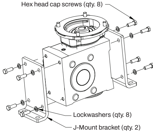
Figure 10 - J-mount Base Kit
