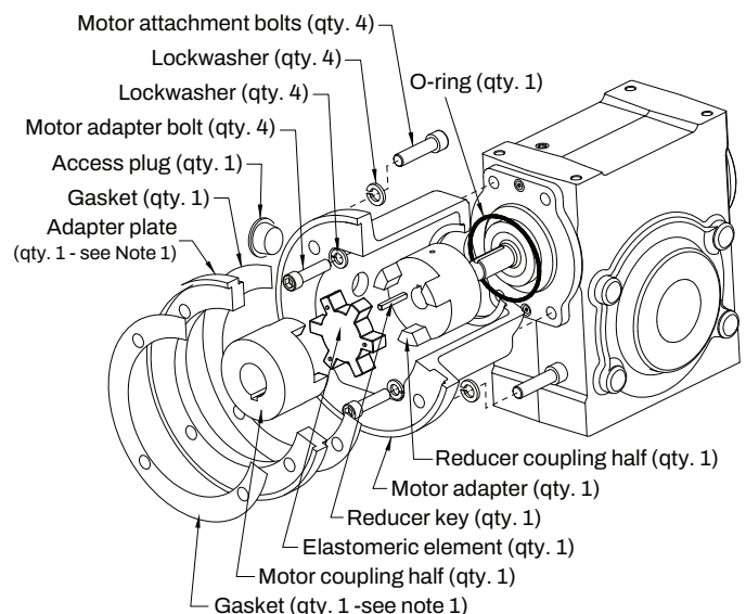
Figure 13 - Motor Adapter Kit
