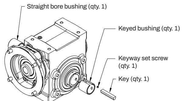
Figure 2 - Straight Bore Bushing Kit
