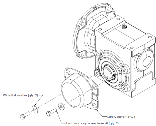
Figure 8 - Installation on non-bearing housing side
