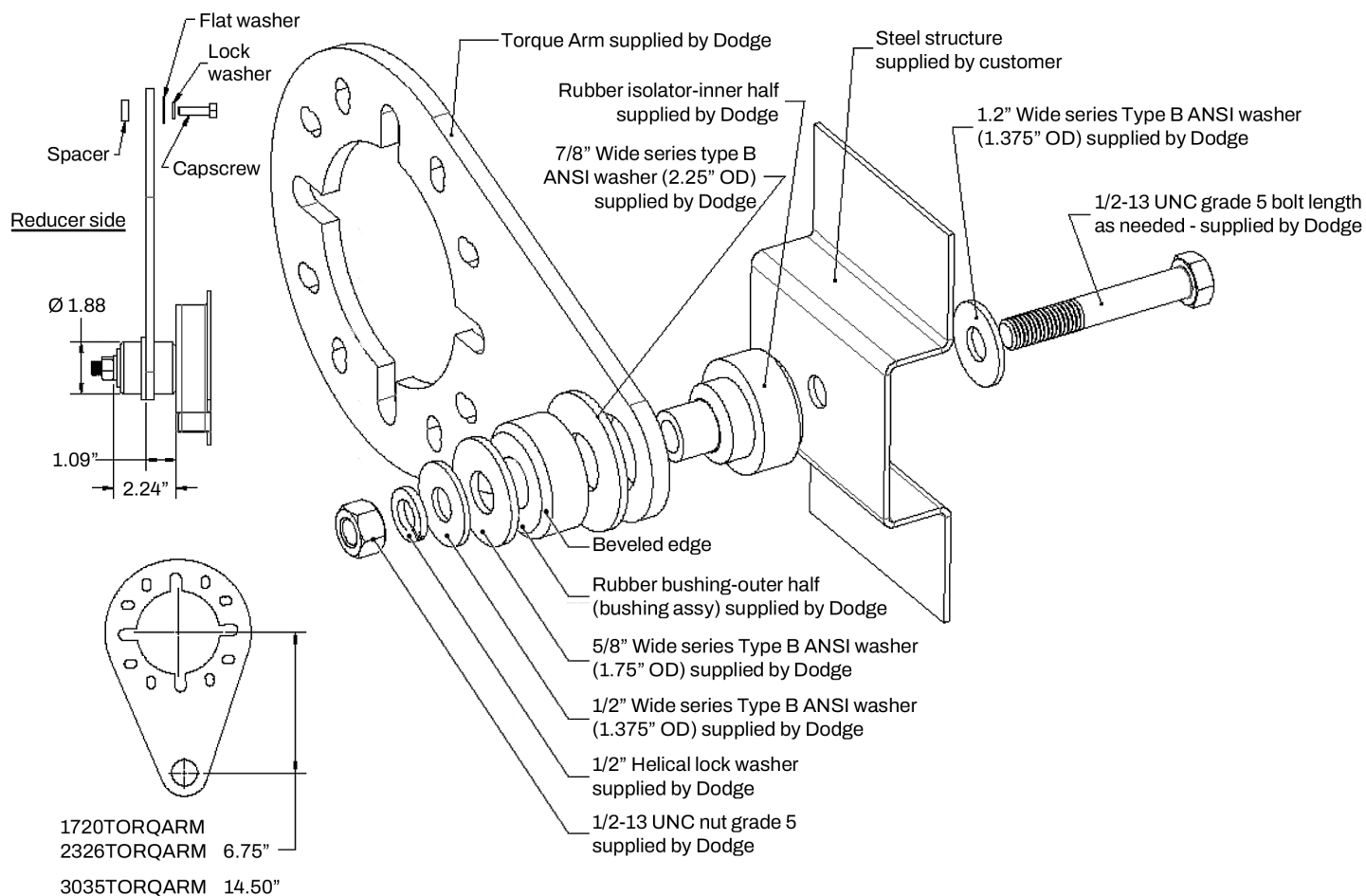
Figure 15 - Banjo Torque Arm Kit
