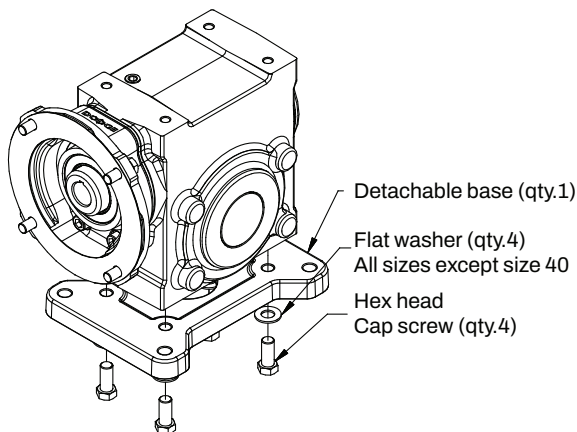
Figure 1 - Bolt-on Base Kit
