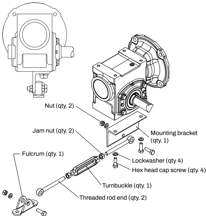
Figure 12 - Tie Rod Kit
