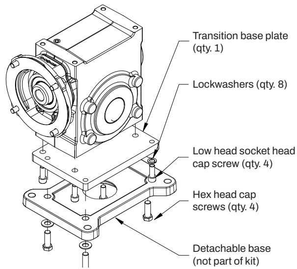
Figure 9 - Transition Kit
