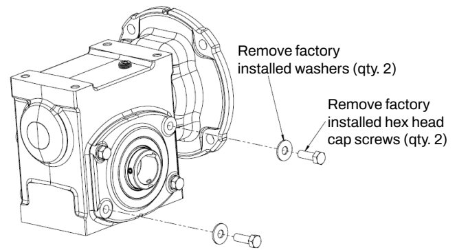
Figure 6 - Factory Screw Removal
