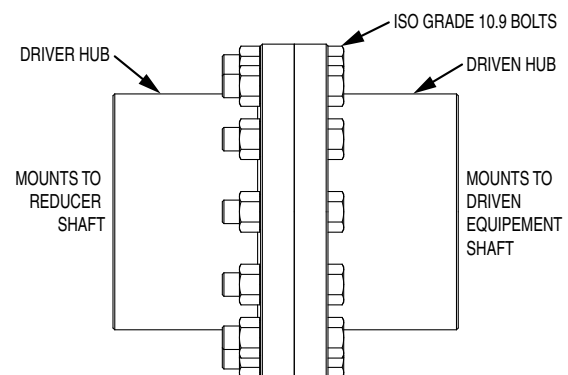
Figure 2 - Coupling Assembly
