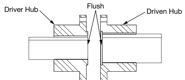
Figure 1 - Hub Installation
