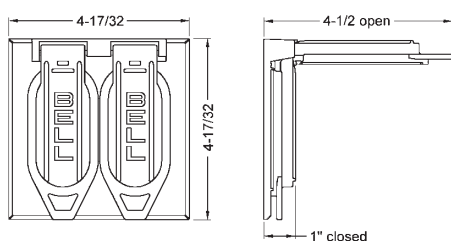
TWO-GANG DEVICE COVERS 5148-0 SERIES, 5096-0, 5160-0, 5098-0
