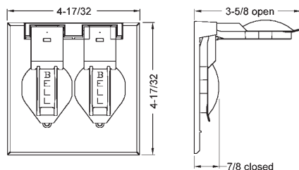
TWO-GANG DEVICE COVERS 5148-0 SERIES, 5096-0, 5160-0, 5098-0
