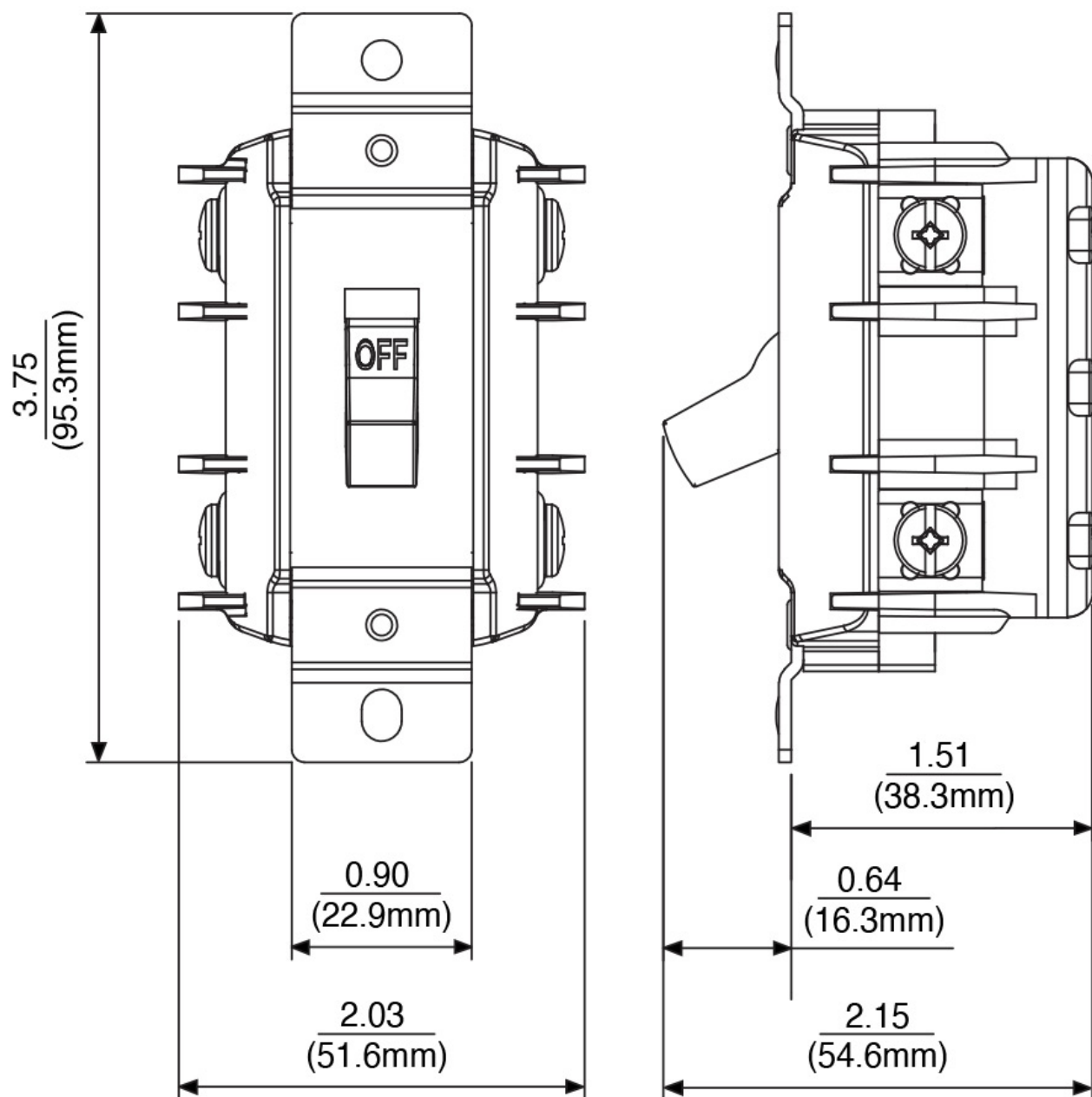
MS302-DSS Shown (Dimensions same for MS303-DSS)
