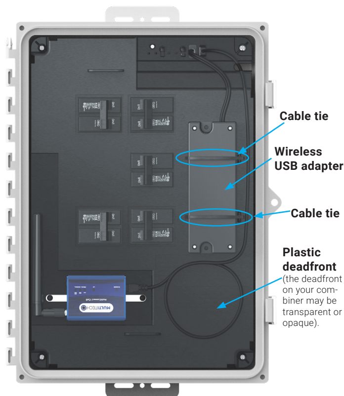
IQ Combiner 3C-ES with Ensemble Communications Kit installed
