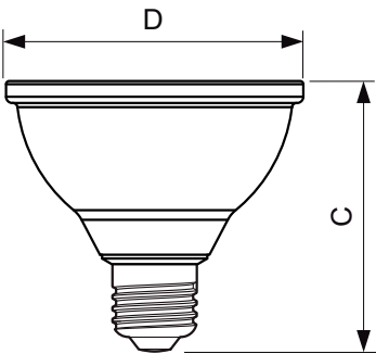
12PAR30S/AMB/F25/830/DIM ULW
