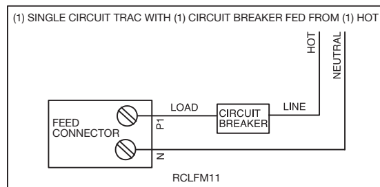
Diagram 1 (End Feed)
