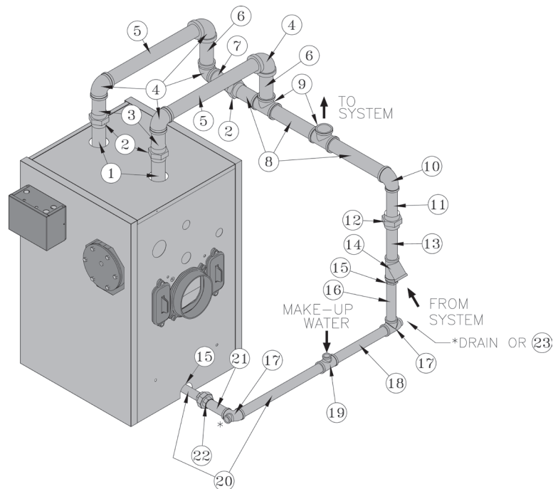
Figure 3: Dropped Header Gravity Return Diagram for MST288, MST396 and MST513
