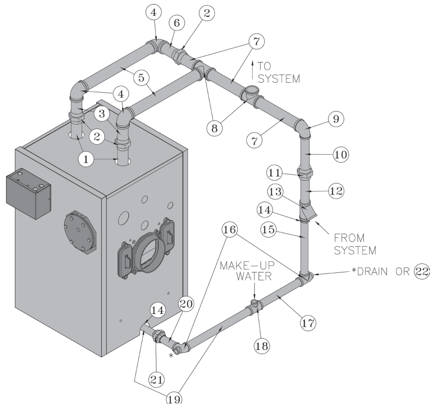
Figure 1: Recommended Gravity Return Diagram for MST288, MST396 and MST513
