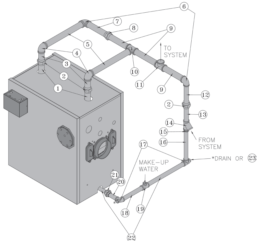
Figure 2: Recommended Gravity Return Diagram for MST629
