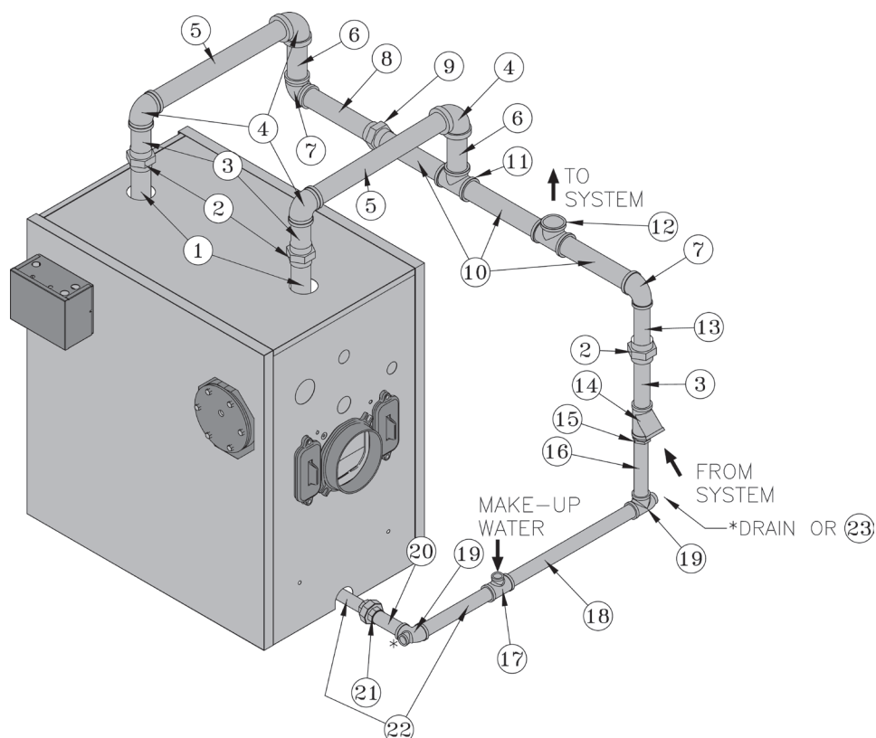
Figure 4: Dropped Header Gravity Return Diagram for MST629
