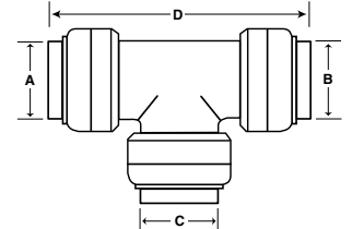
Tee Dimensions
