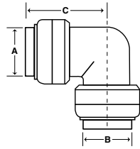
Elbow Dimensions
