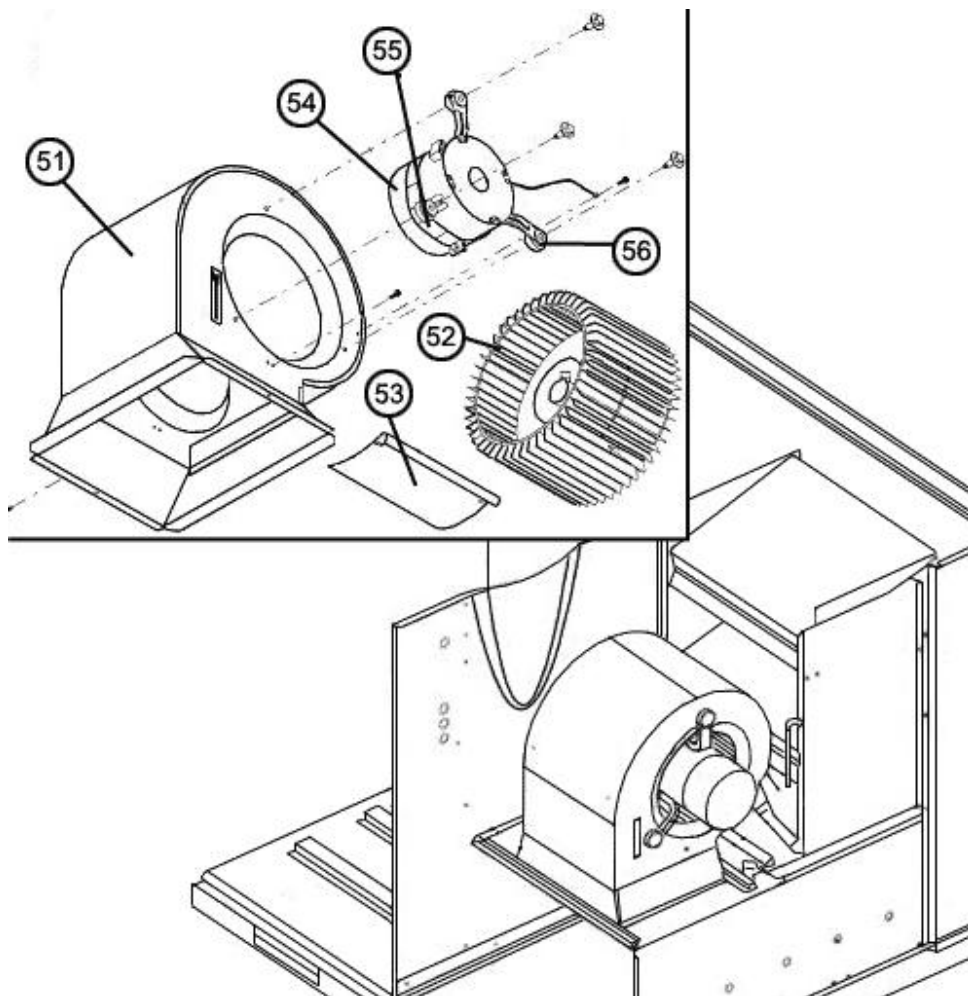
Blower Assembly
