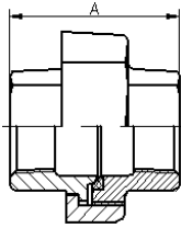
Brass Union
