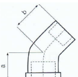
45 Street Elbow
