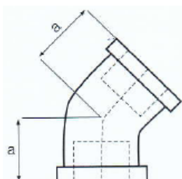
45 Elbow
