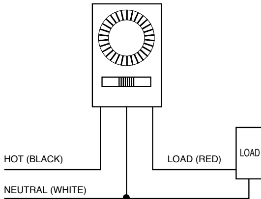
Standard Installation
