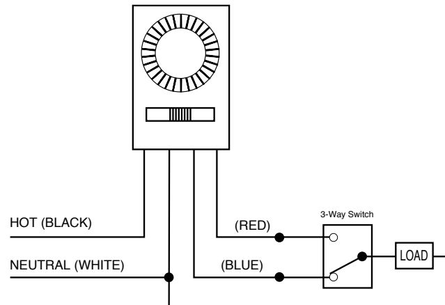
3-Way Installation
