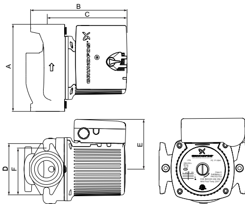
UPS 26-150 F/SF
