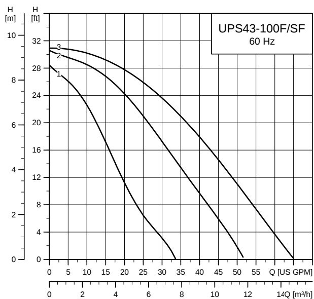
UPS 43-100 F/SF
