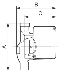
UP 15-18 BUC7
