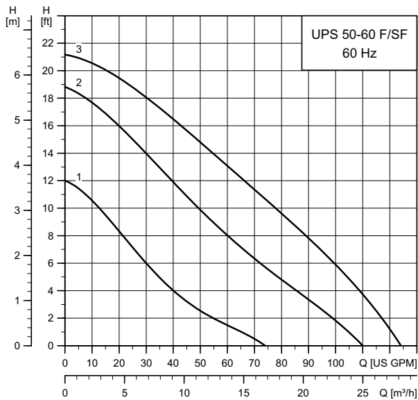
UPS 50-60 F/SF
