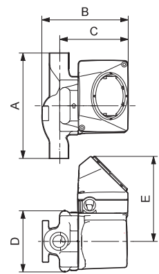
UP 15-18 B7/TLC
