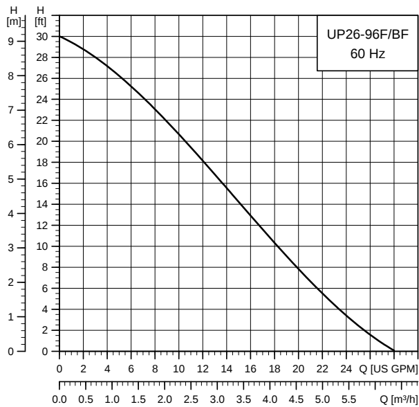
UP 26-96 F
