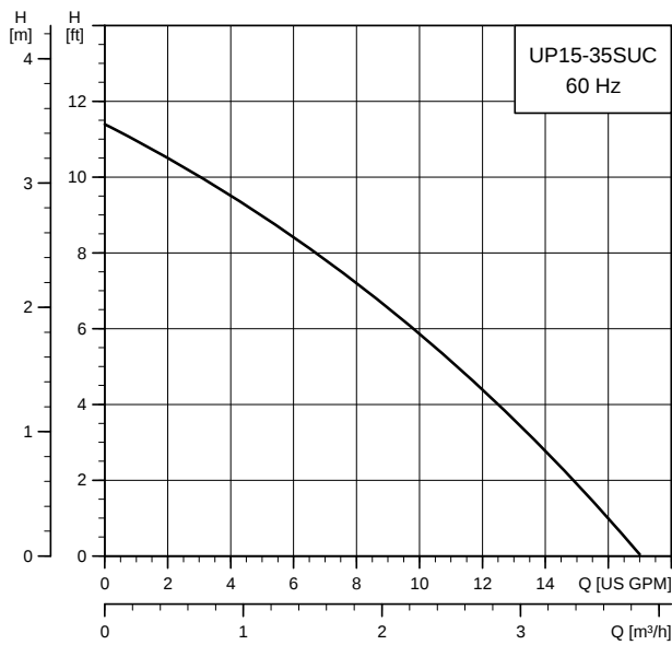
UP 15-35 SUC
