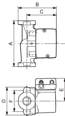
UP 26-96 F
