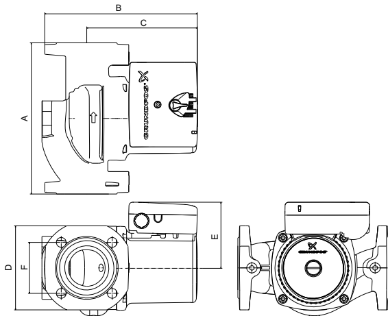
UPS 50-60 F/SF
