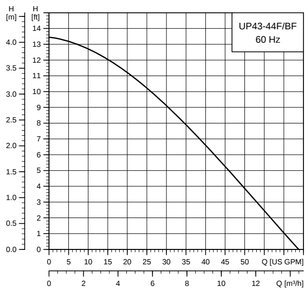
UP 43-44 F/BF
