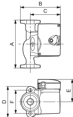
UPS 43-44 FC/BFC
