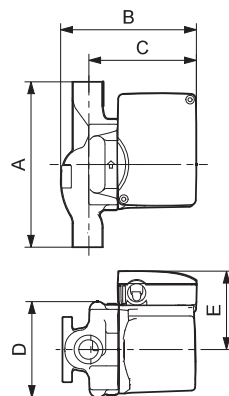
UP 15-18 B7/LC
