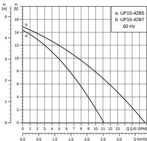
UP 15-42 B5/LC and B7
