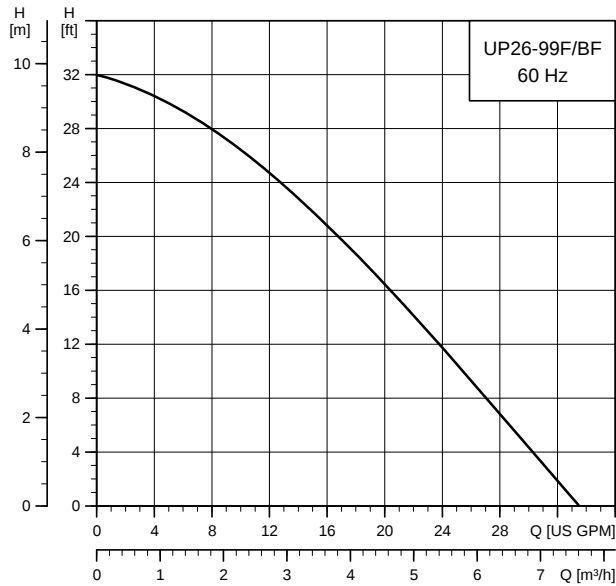
UP 26-99 F/BF
