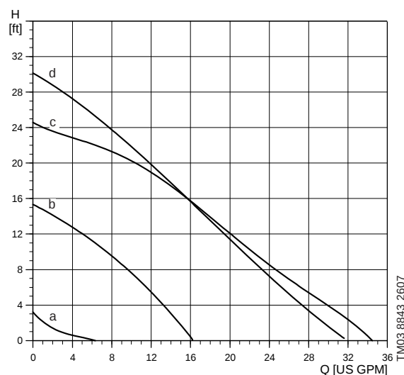
Fig. 6 Family curves for variable-speed pumps
