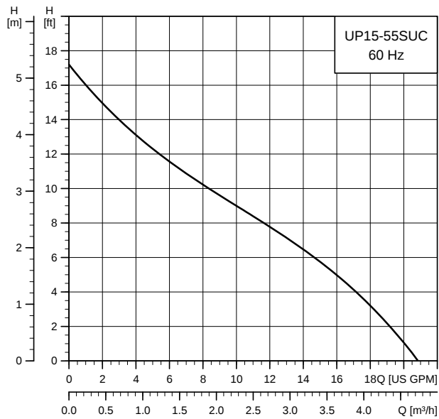
UP 15-55 SUC
