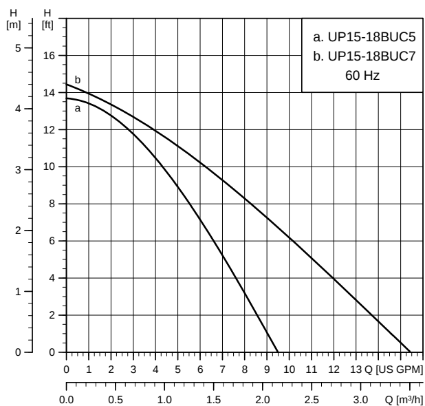
UP 15-18 BUC5
