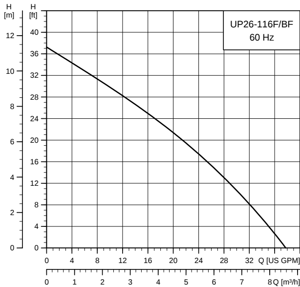
UP 26-116 F
