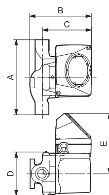
UP 15-42 B7/TLC
