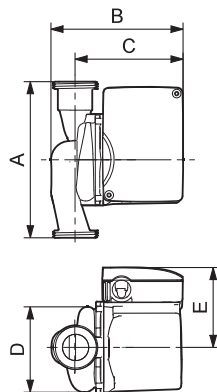
UP 15-55 SUC
