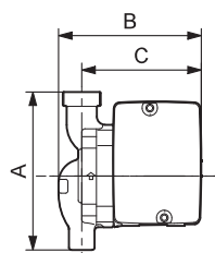
UP 15-42 BUC5/MR
