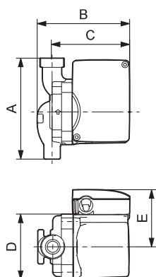
UP 15-10 BUC5 and UP 15-10 BUC5/LC
