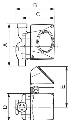
UP 15-10 BUC5/TLC
