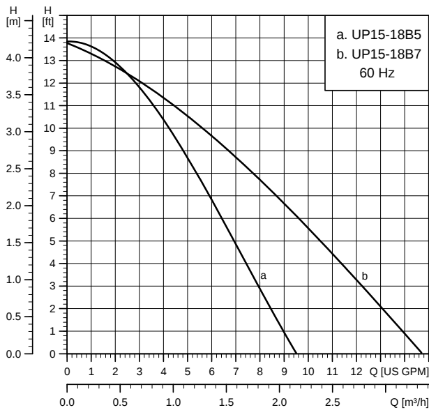
UP 15-18 B5/LC
