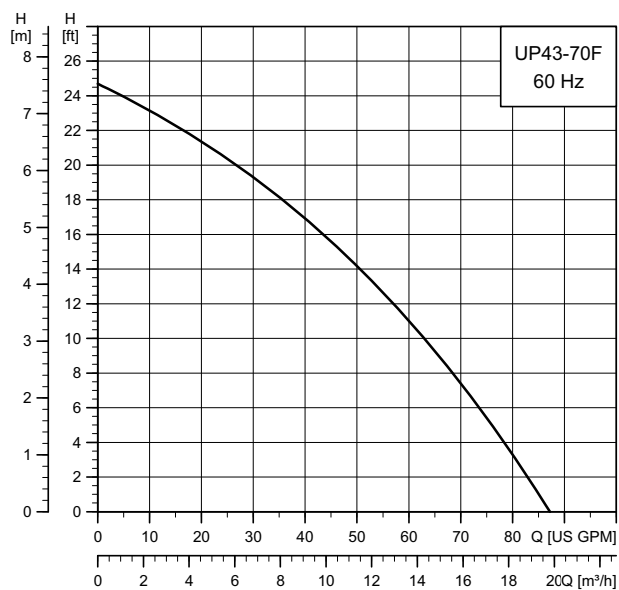
UP 43-70 F
