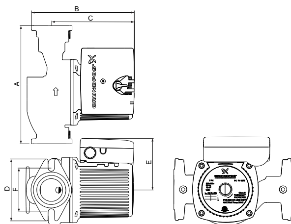
UPS 43-100 F/SF
