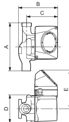
UP 15-10 BUC7/TLC
