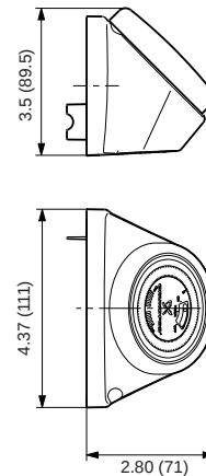
Fig. 13 Timer dimensions, current version
