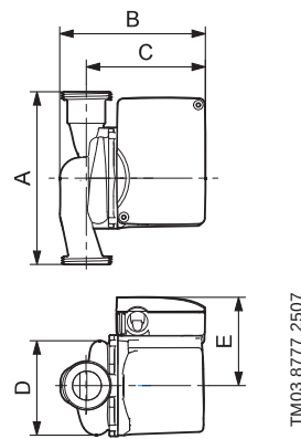
UP 15-29 SU/LC
