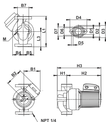
UP 43-70 F
