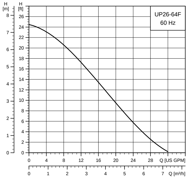
UP 26-64 F
