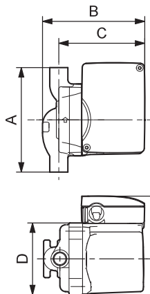
UP 15-10 B5 and UP 15-10 B5/LC
