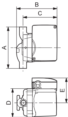
UP 15-18 B5/LC
