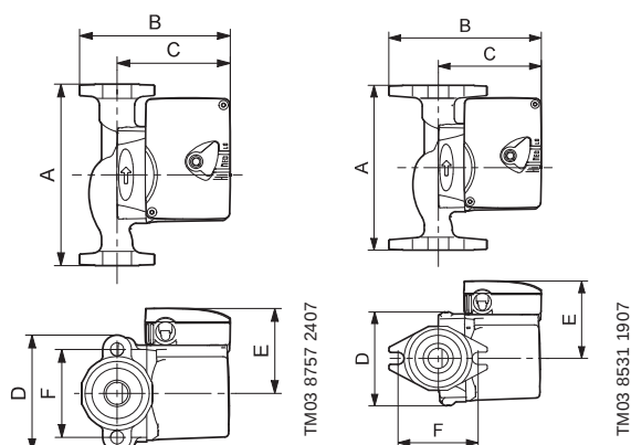
UPS 26-99 FC
