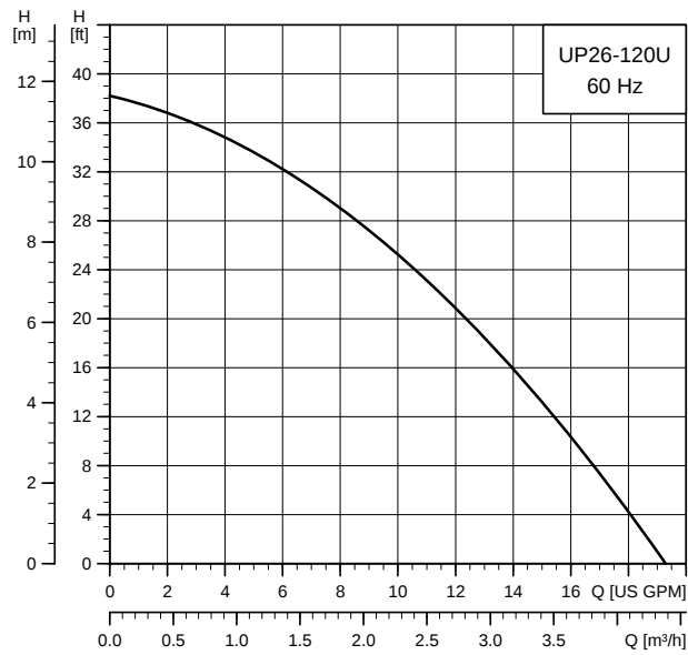
UP 26-120 U
