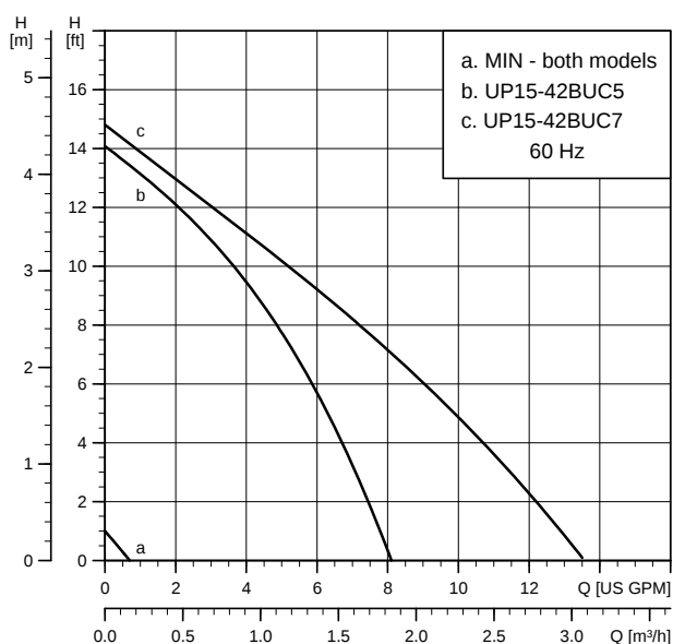
UP 15-42 BUC5/MR
