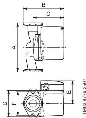
UP 15-29 SF
