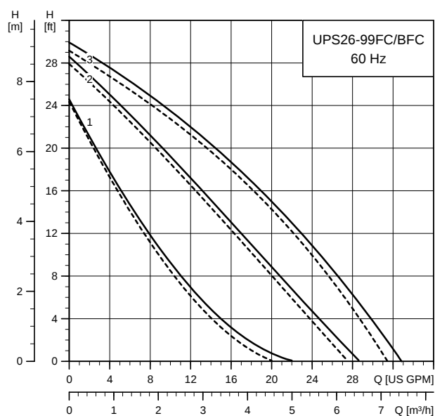
UPS 26-99 FC
