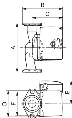
UPS 15-35 SFC
