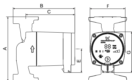
ALPHA 15-55 F Linecord
