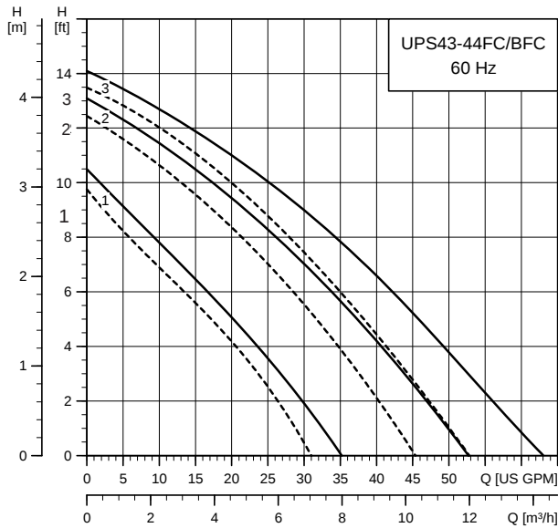
UPS 43-44 FC/BFC
