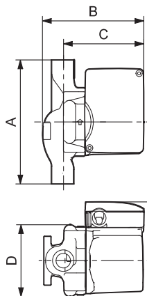
UP 15-10 B7 and UP 15-10 B7/LC
