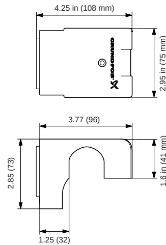
Fig. 12 Timer dimensions, previous version
