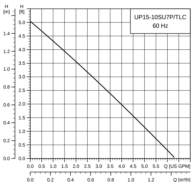
UP 15-10 SU7P/TLC
