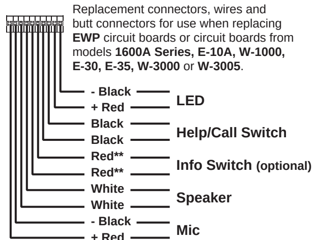
FIGURE 1 Replacement Cable Assembly (included)
