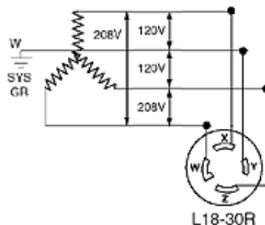
Wiring Diagram
