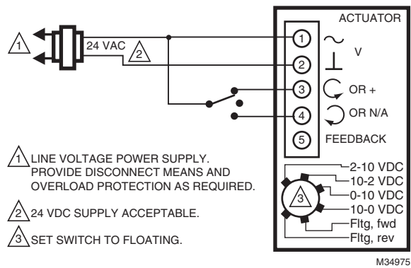
Fig. 11. MS7505 with Floating Control (Floating mode setting).
