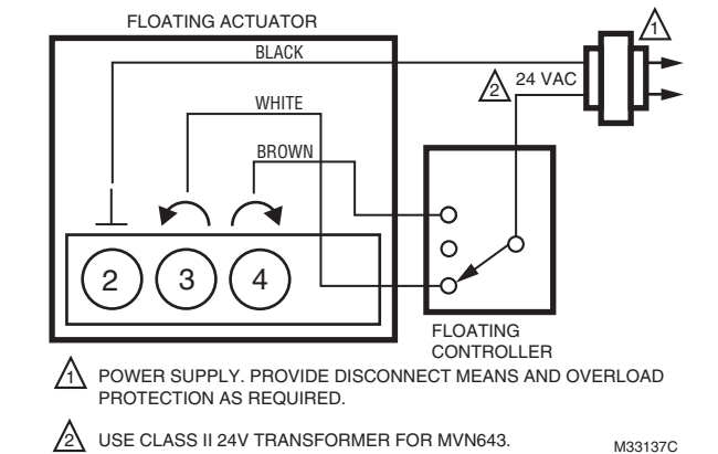
Fig. 16. MVN613 or MVN643 with Floating Control.
