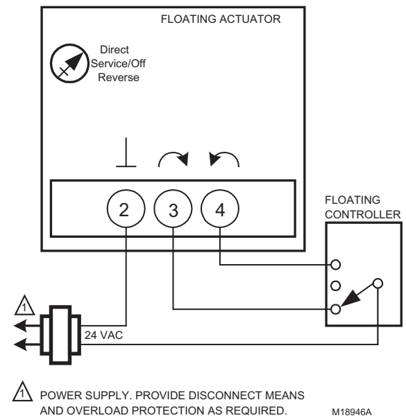
Fig. 8. MN6105 with Floating Control.
