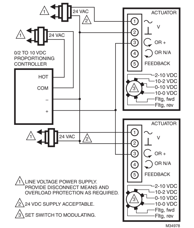
Fig. 15. MS7505 with Proportioning controllers operating multiple actuators (Modulating mode setting).
