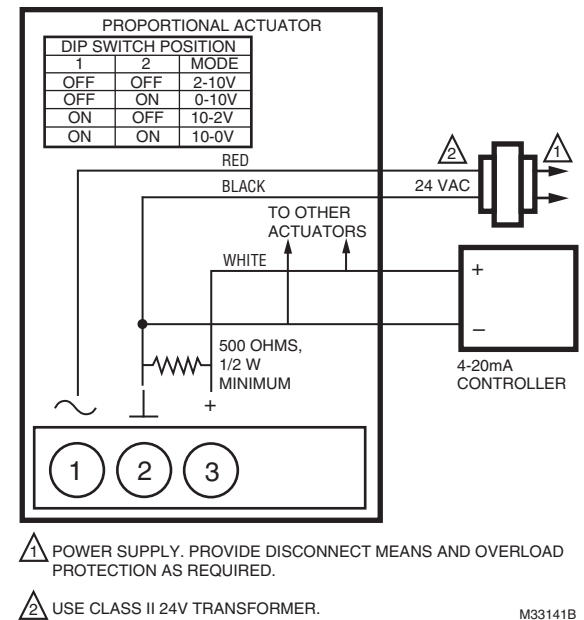
Fig. 19. MVN713 with 4-20mA Control.
