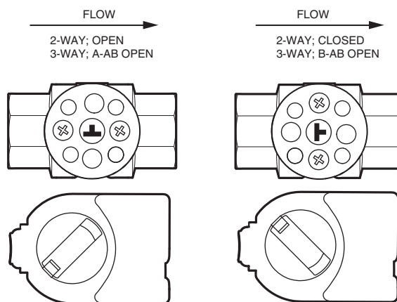
Fig. 1. Three-way ball valve flow orientation (not to scale).
