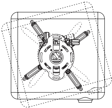
SWIVEL (YAW) 360° (when attached to extension column) +/- 15° (when flush mounted)
