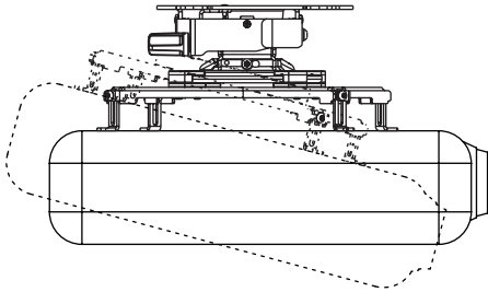
+15/- 20° PITCH
