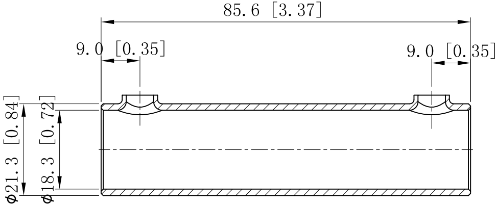
CUTAWAY VIEW A-A
